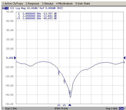
Return Loss
